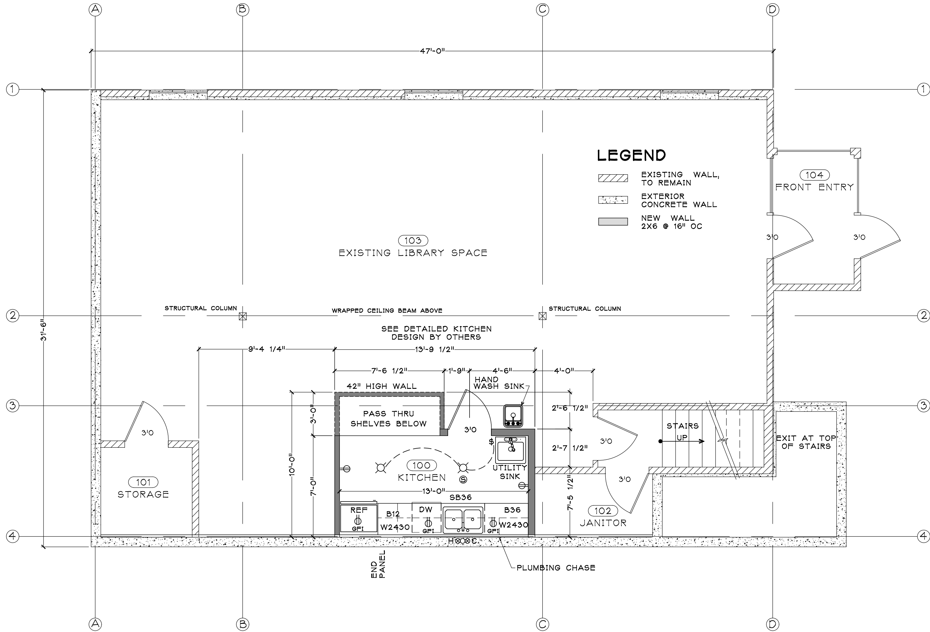
PROPOSED KITCHEN PLAN 1/4" = 1'-0"
